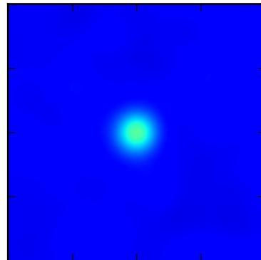
Gaussian2DKernel
