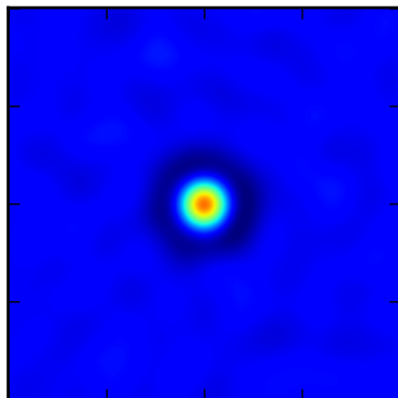
MexicanHat2DKernel
