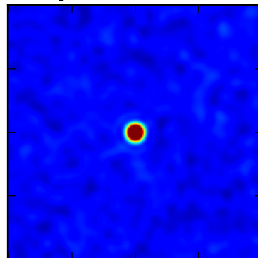
AiryDisk2DKernel
