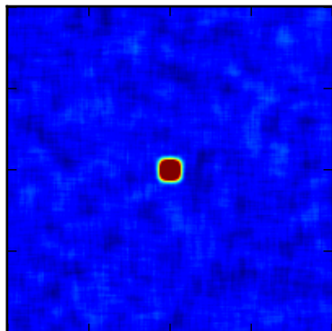
Box2DKernel
