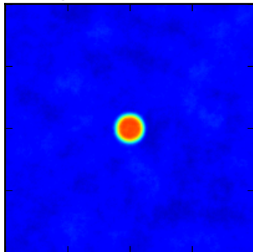
Tophat2DKernel
